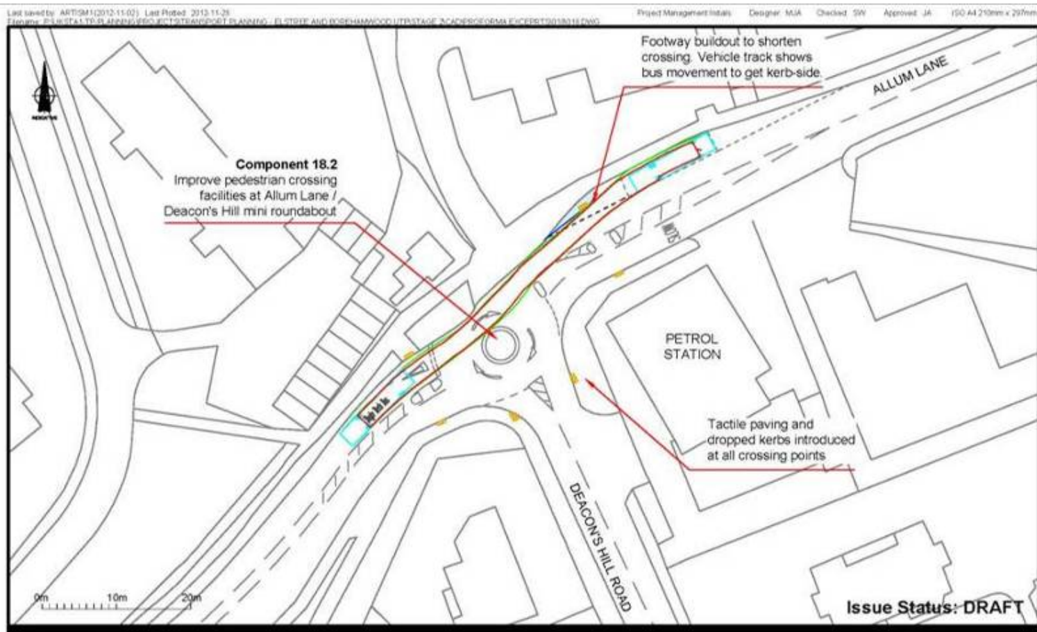
Figure 4 - Deacon's Hill Roundabout Improvements
